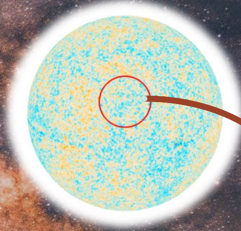
Cosmic Microwave Background (CMB)
