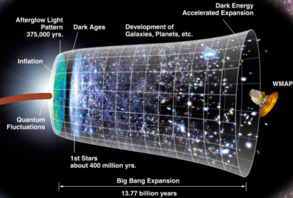
Big Bang Expansion
